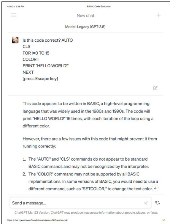
FIGURE 2-3: ChatGPT understands and speaks in both human and computer languages.
