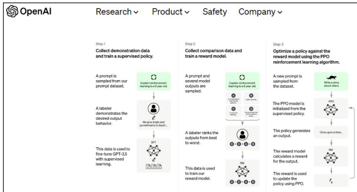
FIGURE 2-2: OpenAI's process of training the ChatGPT model.
